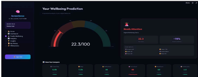
Fig. 6. Prediction Page
