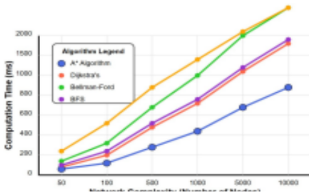
Fig. 2. Algorithm Comparison of ScreenSense
